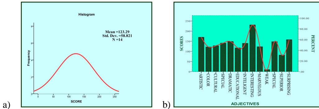
Figure no. 3 The frequencies histogram; b) The absolute frequencies bar graphical representation(SPSS)
