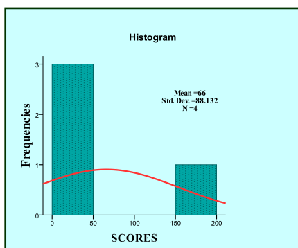
Figure no. 12 The frequencies histogram
