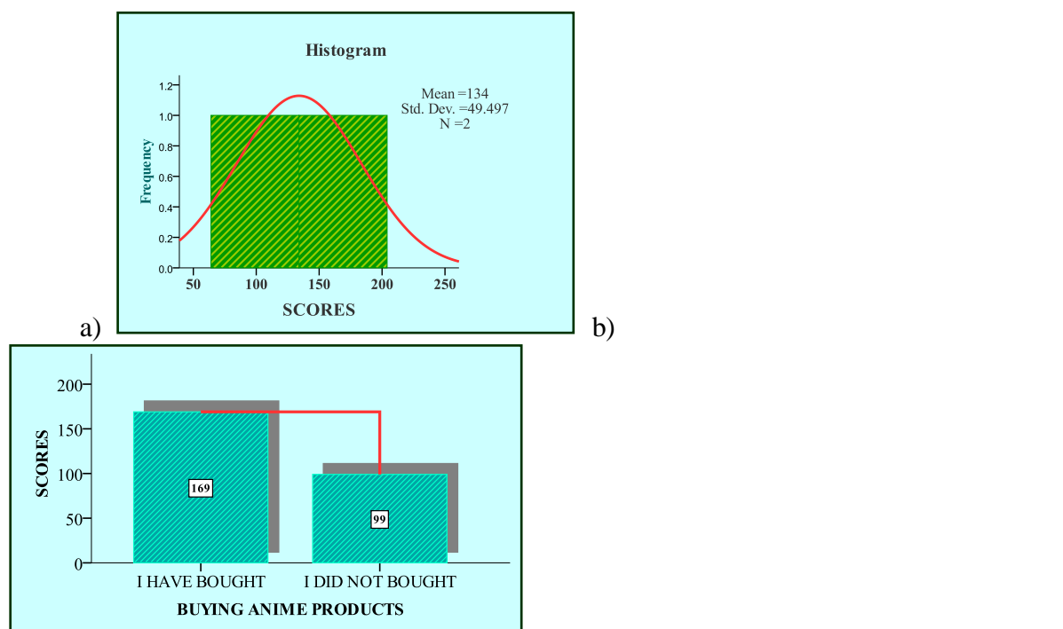
Figure no. 5 The frequencies histogram; b) The absolute frequencies bar graphical representation(SPSS)
